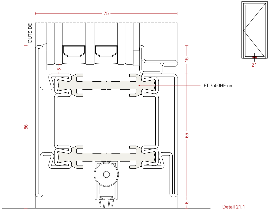
Detail 21.1
