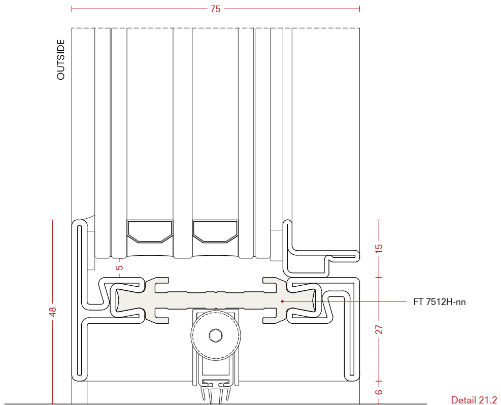
Detail 21.2
