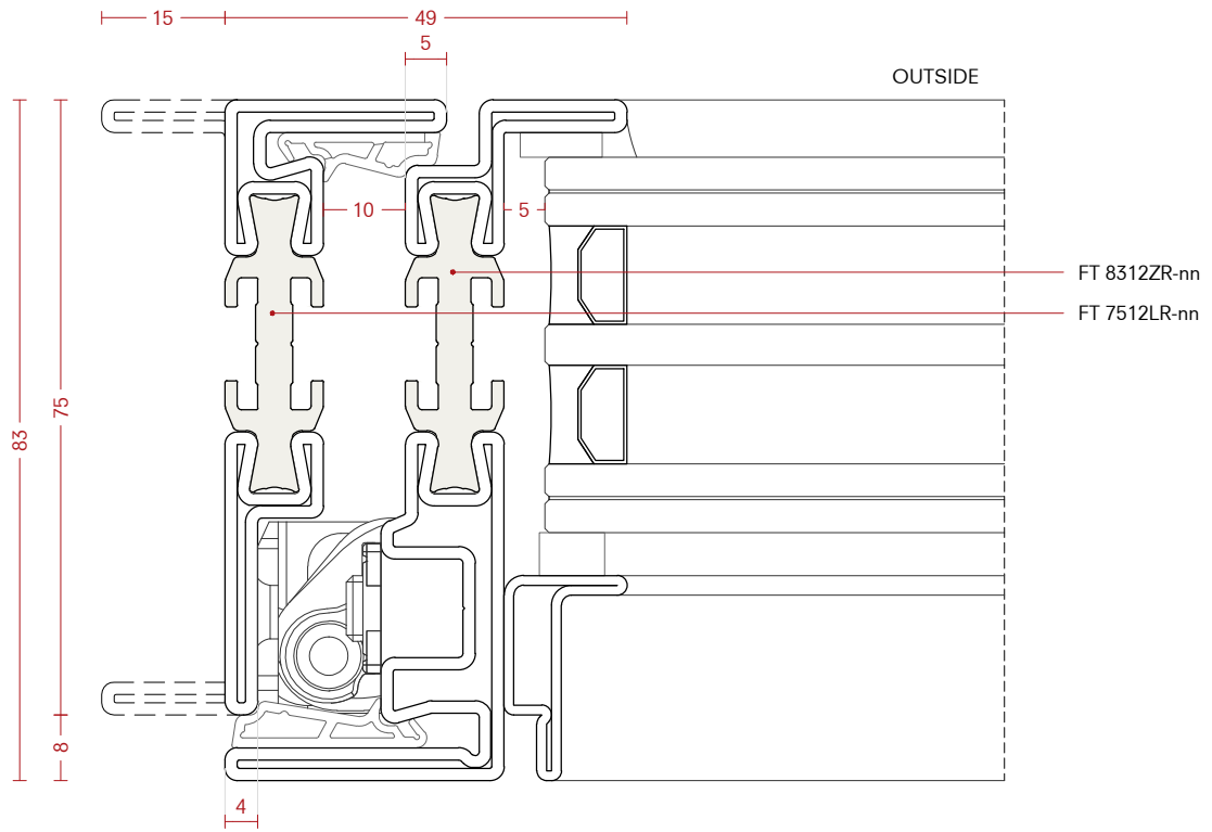
Detail 4.3
