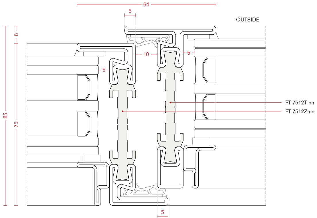
Detail 10.2
