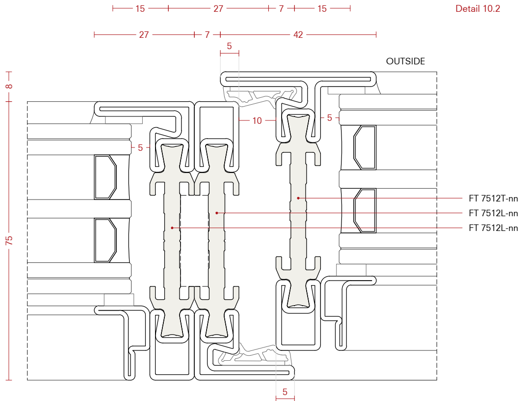
Detail 11.2
