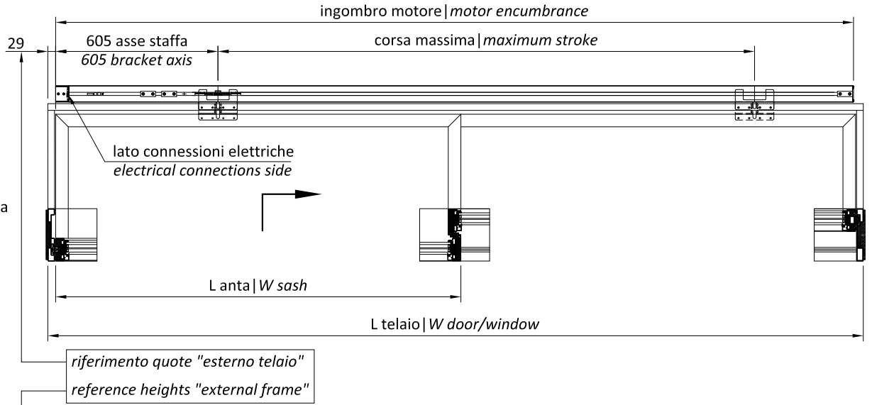
Schema | Type B*
