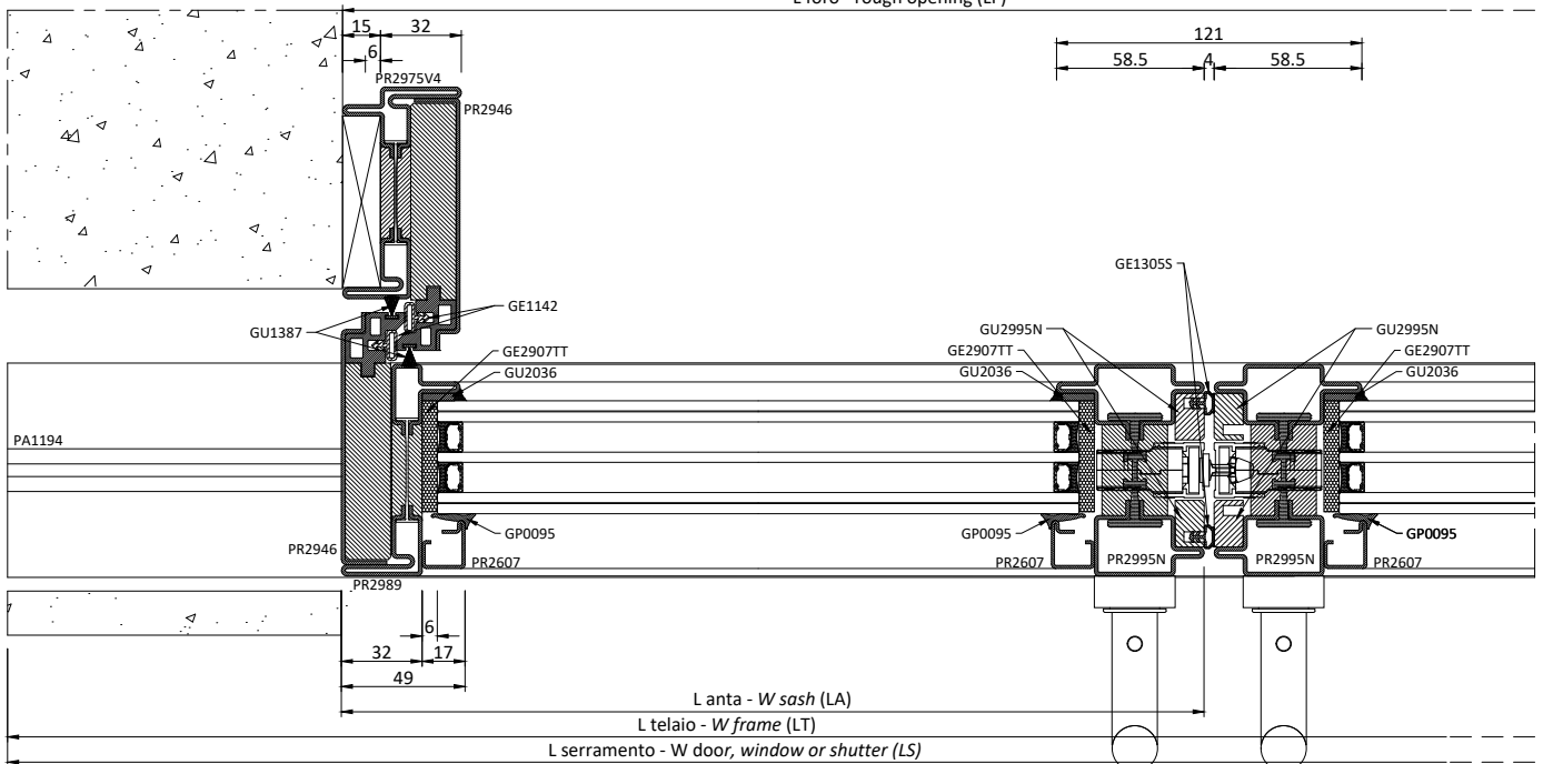
L foro - rough opening (LF)
