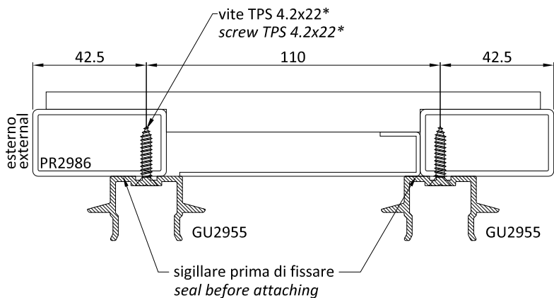
Schema | Type F
