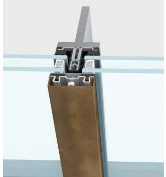
application to mullion | 50 mm face section
